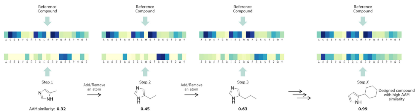
Figure 2. Atom-based generation modifies molecular structures iteratively while assessing similarity to the reference AAM profile
