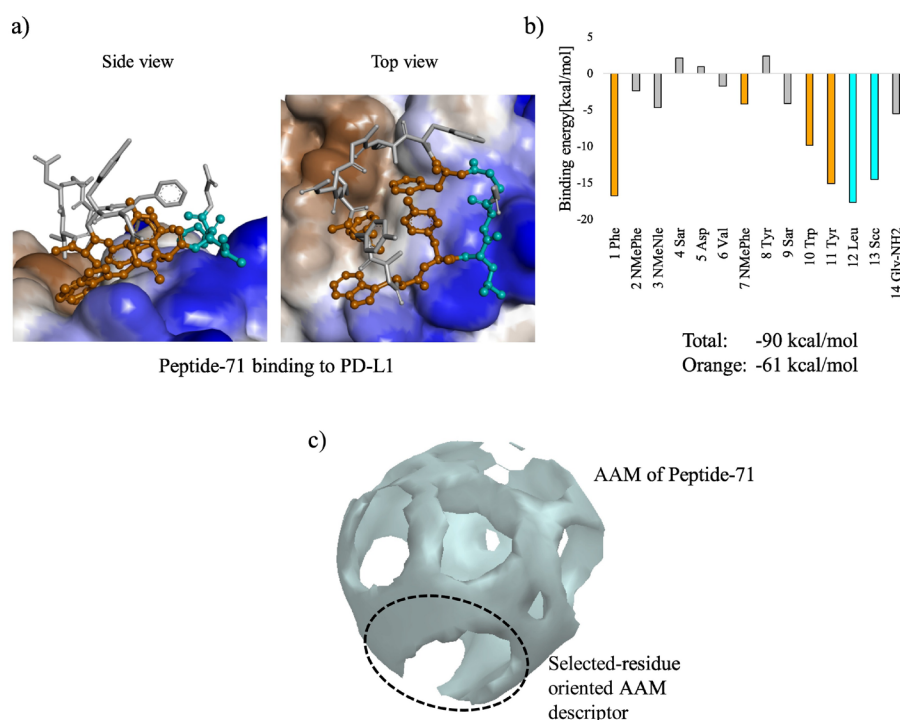
Figure 4. (a) Peptide-71 in the PD-L1 binding site. (b) FMO-derived residue interaction-energy contributions. (c) Selected-residue AAM descriptor derived from the localised peptide region chosen for small-molecule translation
